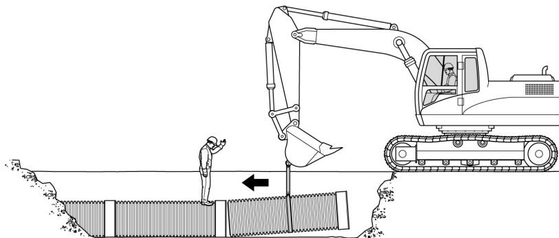
Figure 11: Installing Large Diameter Pipe with Sling
