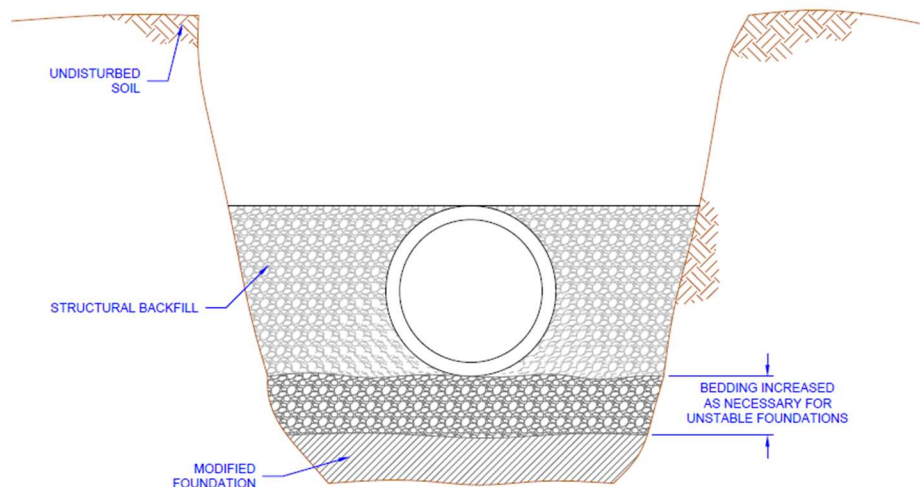
Figure 5: Modified Foundation
