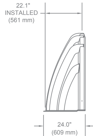
HydroStor® HS180 end cap side view
